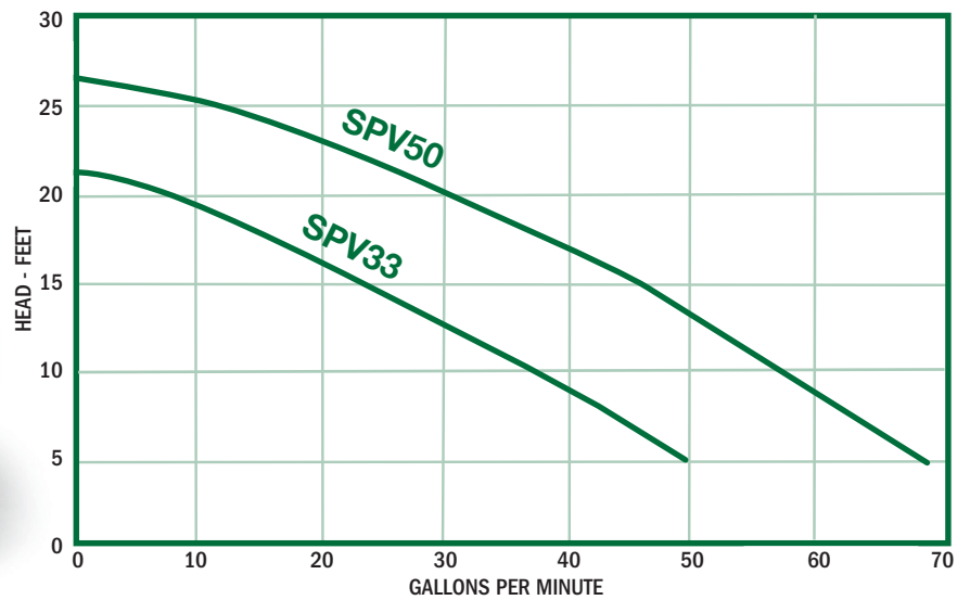
Performance Curve
